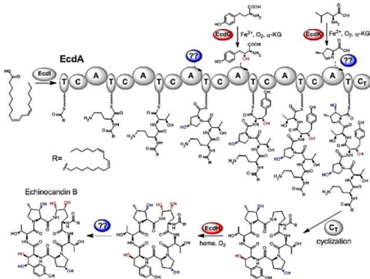
Figure 6. Proposed timing of post-translational hydroxylations for biosynthesis of echinocandins B (1). Confirmed steps and modifications are highlighted in red, while proposed ones are in blue.
